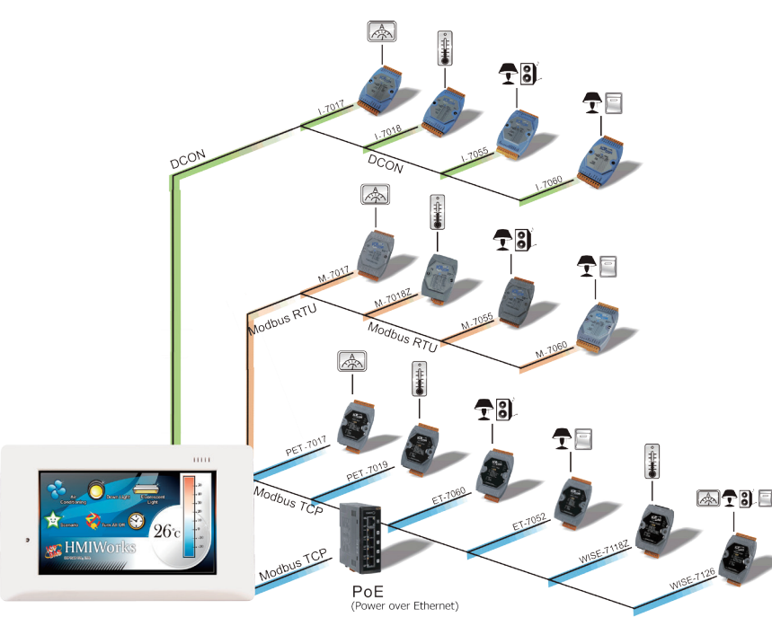
TPD-433F-H with External Wall Box EWB-T43F
