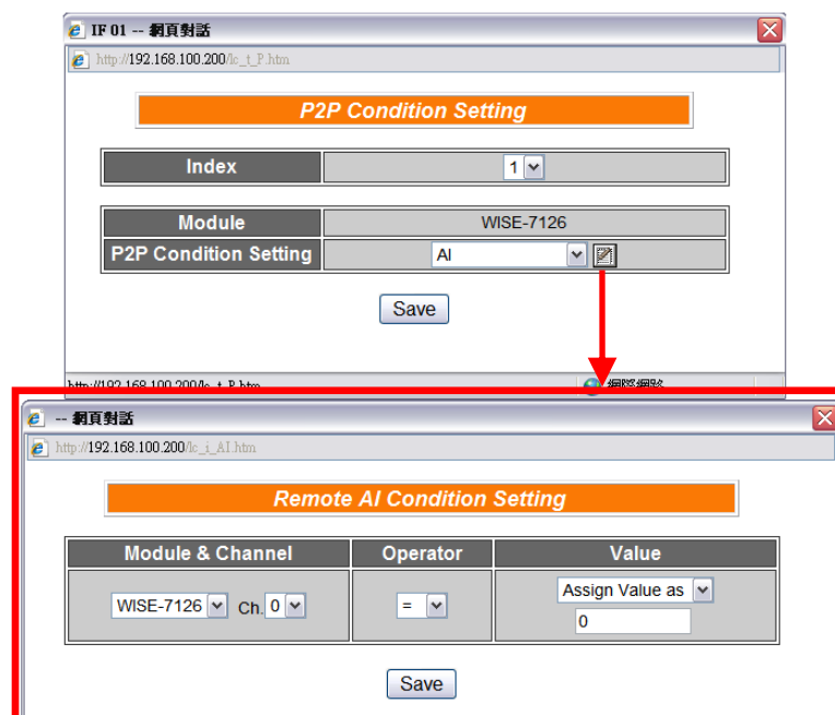
Figure 6-12 : P2P IF Condition detail setting page
