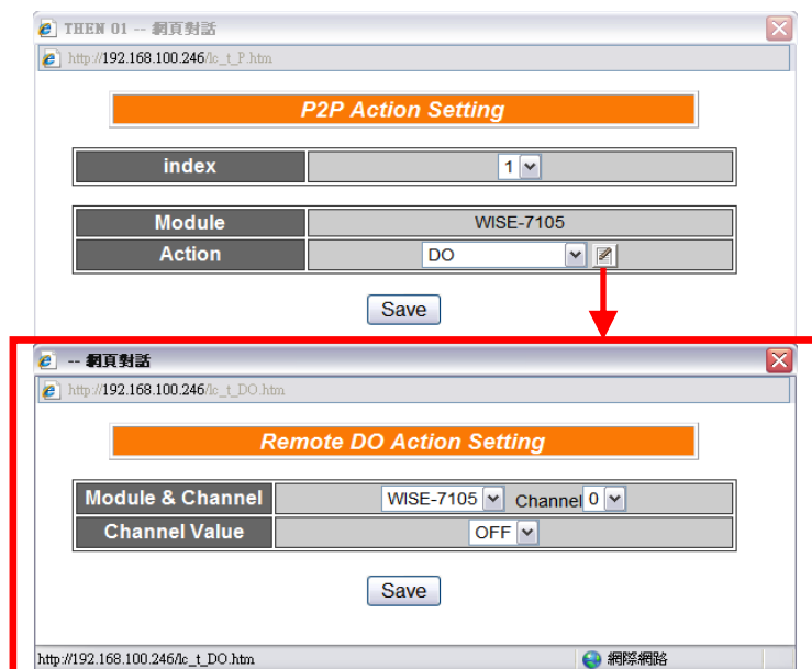
Figure 6-26 : P2P action detail setting page
